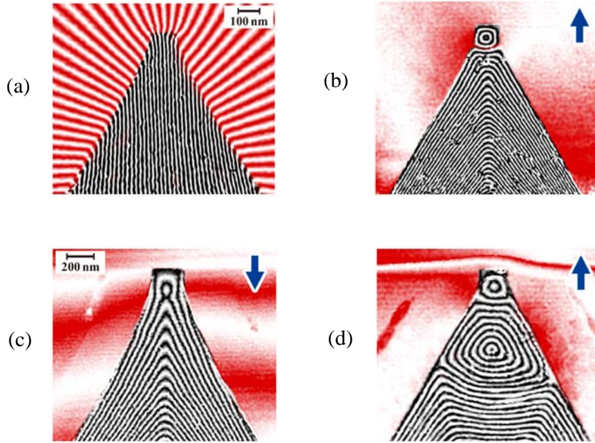
FIG. 1. Interference micrographs showing magnetic lines of force of magnetic heads for perpendicular recording: (a) H = 80 Oe (NiFe); (b) H = 0 (NiFe) after the upward magnetic field; (c) H = 0 (NiFe) after the downward magnetic field; (d) H = 0 (CoNiFe).
