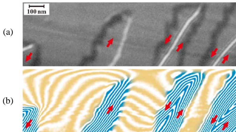
FIG. 2. Growth of ferromagnetic domains in colossal magnetoresistance manganite, \text{La}_{0.25}\text{Pr}_{0.375}\text{Ca}_{0.375}\text{MnO}_3 , thin film at T = 62.4 K: (a) Lorentz micrograph; (b) interference micrograph.
